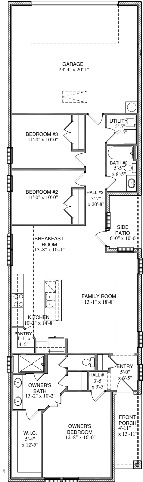
FLOOR PLAN
