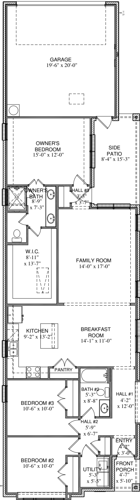
FLOOR PLAN
